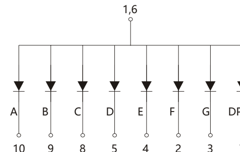
Common Anode JS1-3012Bx
