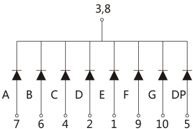
Common Cathode JS1-5611Ax
