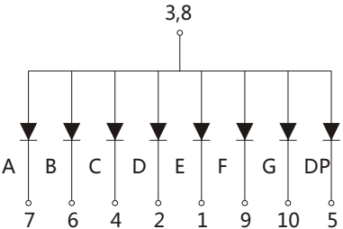
Common Anode JS1-5611Bx
