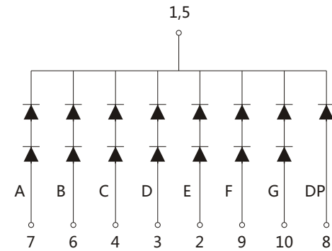
Common Anode JS1-15011Bx
