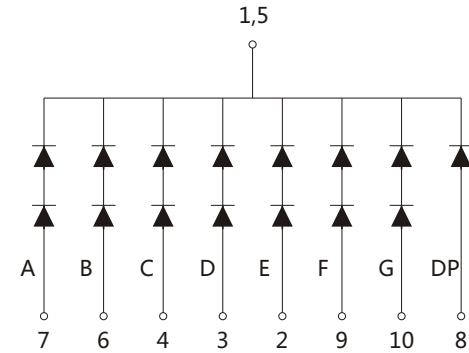
Common Anode JS1-15013Bx
