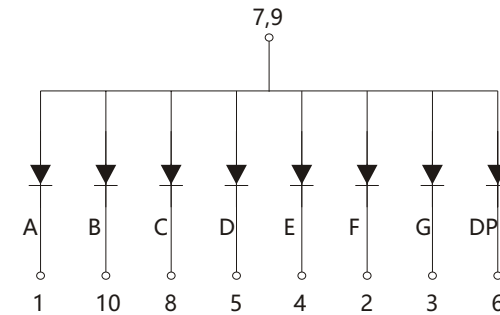
Common Anode JSD-3211Dx
