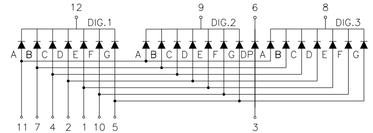
Common Anode JSD-4031Hx
