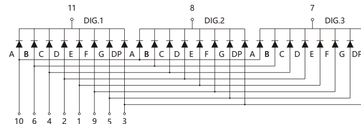
Common Anode JSD-4031H2x
