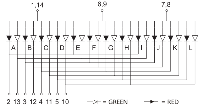
Common Anode JSD-123010Bxx
