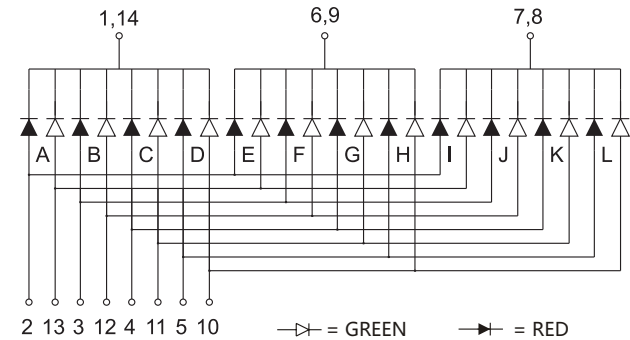
Common Cathode JSD-123010Axx
