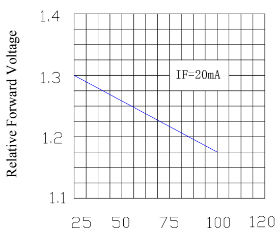
Forward Voltage & Ambient Temperature(°C)
