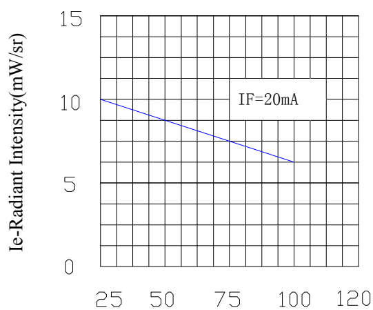
Relative Intensity & Ambient Temperature(°C)
